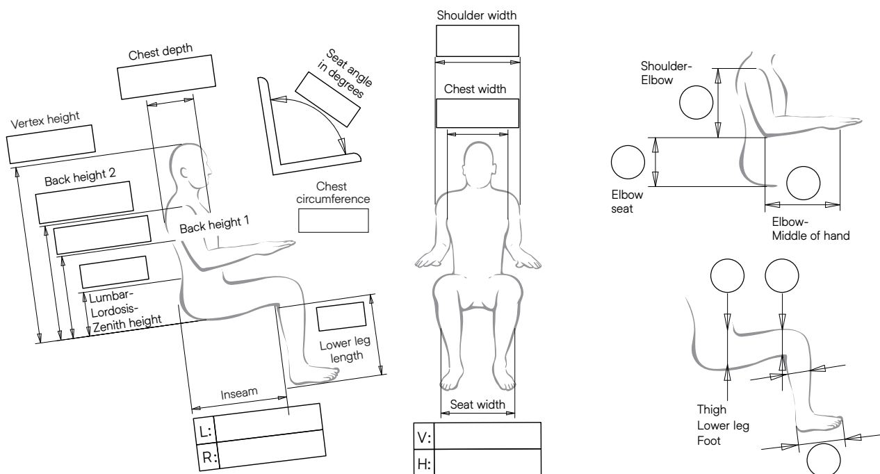
Measurement sheet / Seat dimensions
